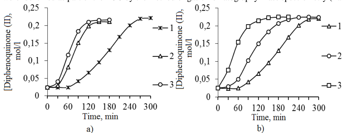
Fig. 3. Kinetic curves of accumulation in DPQ during the MP oxidation reaction in toluene according to the composition of the catalyst system. The catalyst concentration of [\text{KOH}] = 16 \text{ mol/l} in a KOH solution in the reaction mixture - 3.0% by weight.: a: 1 - without DMSO, 2 - [\text{DMSO}] = 0.5\% \text{ by weight} , 3 - [\text{DMSO}] = 1.0\% \text{ by weight} . b: 1 - without \text{DMSO}_2 , 2 - [\text{DMSO}_2] = 1.0 \text{ wt}\% , 3 - [\text{DMSO}_2] = 2.0 \text{ wt}\% .
