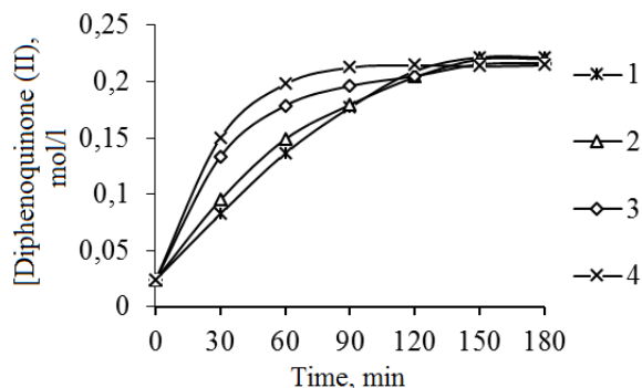
Fig. 2. Kinetic curves of DPQ accumulation during MP oxidation reaction in toluene dependent on concentration of POC catalyst: 1 - [\text{POC}] = 3.0 \text{ wt}\% , 2 - [\text{POC}] = 4.4 \text{ wt}\% , 3 - [\text{POC}] = 7.1\% \text{ mass} , 4 - [\text{POC}] = 13.3\% \text{ wt} .
