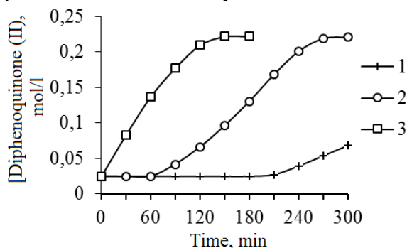
Fig. 1. The kinetic curves of DPQ accumulation during MP oxidation reaction in toluene in the dependence on the type of catalyst: 1 - [\text{KOH}] = 6.8 \text{ mol/l} ; 2 - [\text{KOH}] = 16 \text{ mol/l} ; 3 - POC ( [\text{KOH}] = 6.8 \text{ mol/l} )
