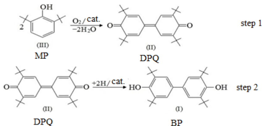
Figure 1. A two-step process of the BP synthesis.
