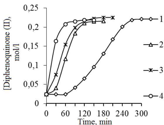
Fig. 4. Kinetic curves of DPQ accumulation during the oxidation reaction of MP in toluene according to the composition of the catalyst system. The catalyst concentration of [16 mol/l] aqueous KOH solution in the reaction mixture - 3.0% wt.: 1 - idle; 2 - [DMSO] = 1.0% wt.; 3 - [DMSO 2 ] = 2.0% wt.; 4 - [DMSO] = 1.0% by weight. + [DMSO 2 ] = 2.0 wt%.
